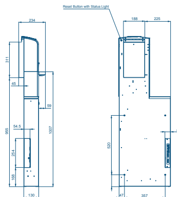
Coin Recycler – Tall
