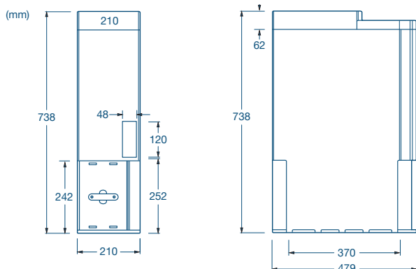
Note Recycler with Interface Cassette
