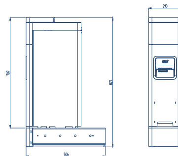
Coin Recycler Slim
