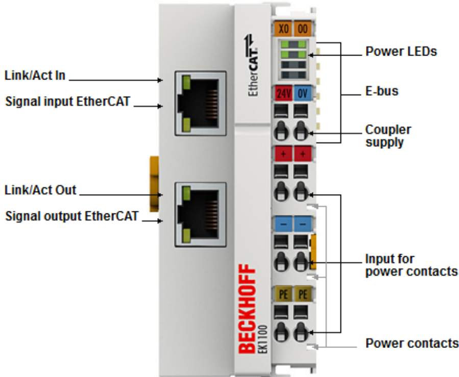
Abb. 5: EK1100
