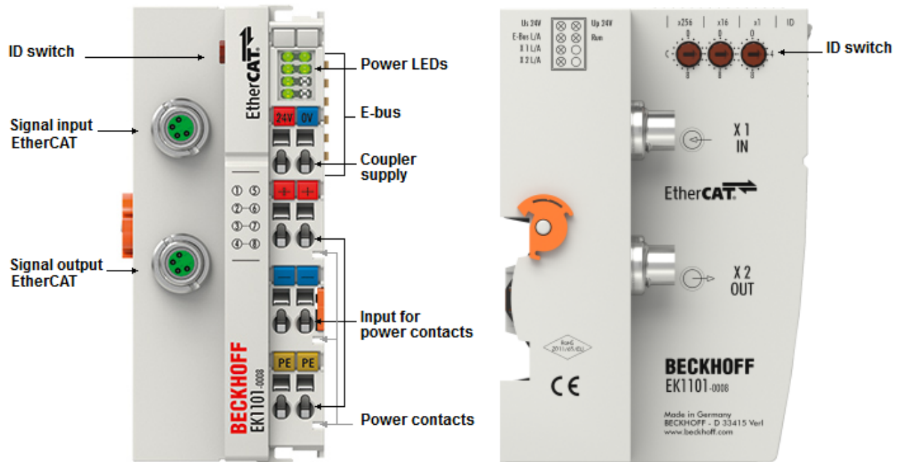
Abb. 19: EK1101-0008
