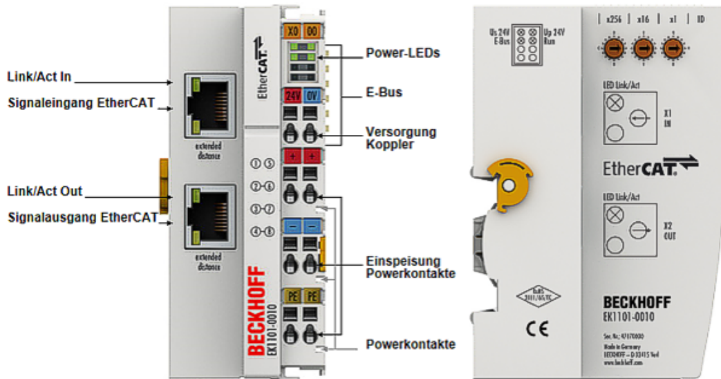
Abb. 7: EK1101-0010
