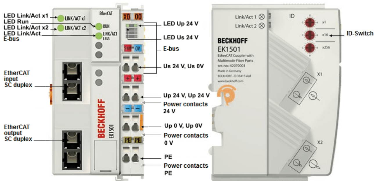
Abb. 48: EK1501
