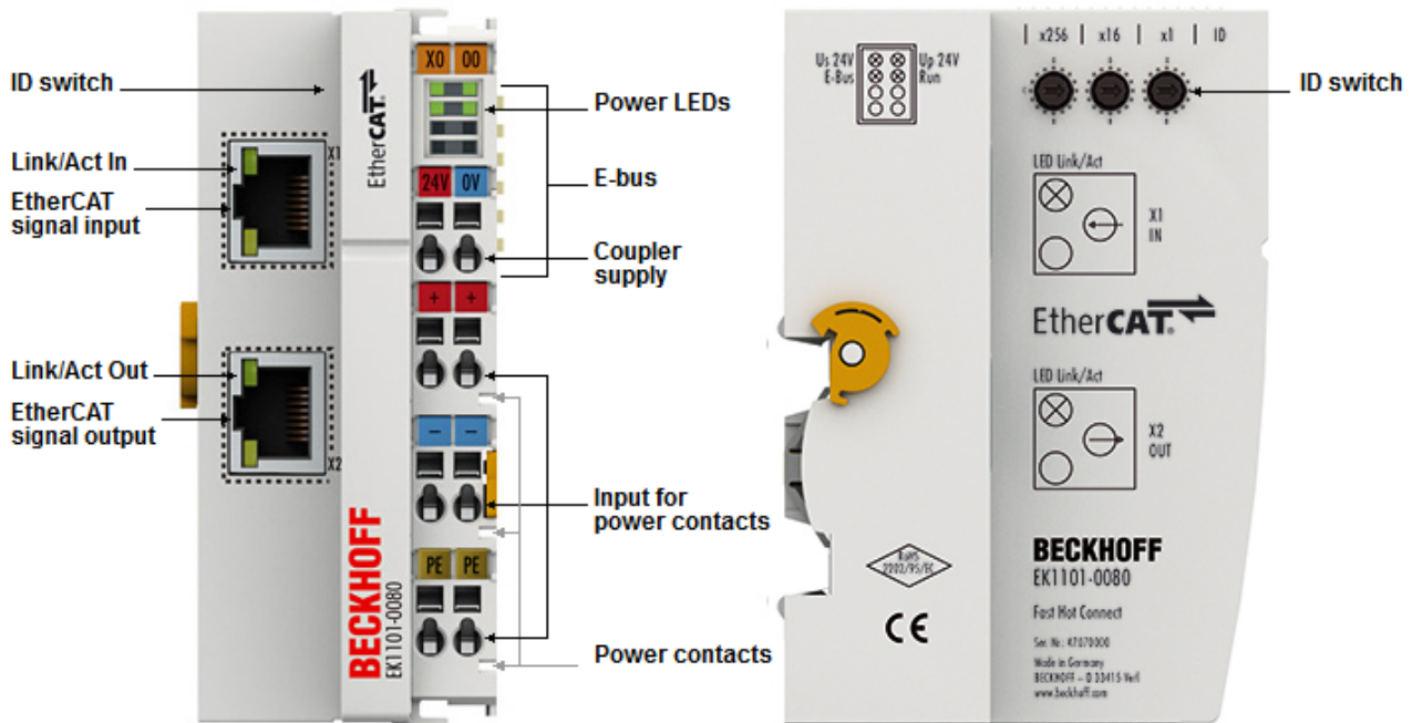
Abb. 11: EK1101-0080
