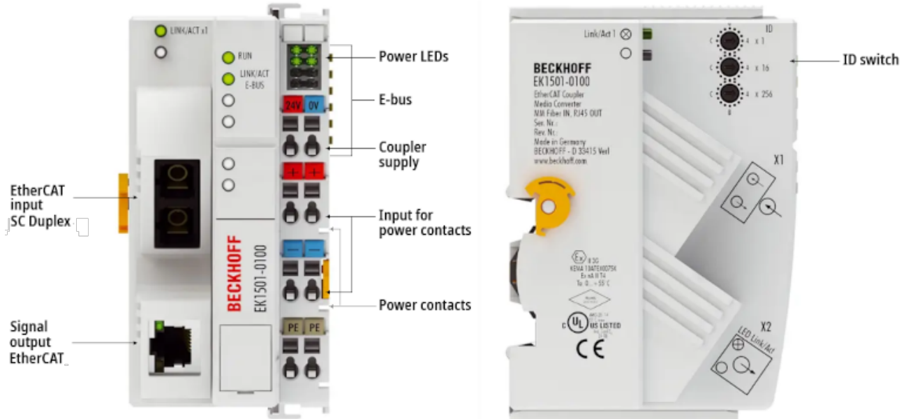
Abb. 22: EK1501-0100
