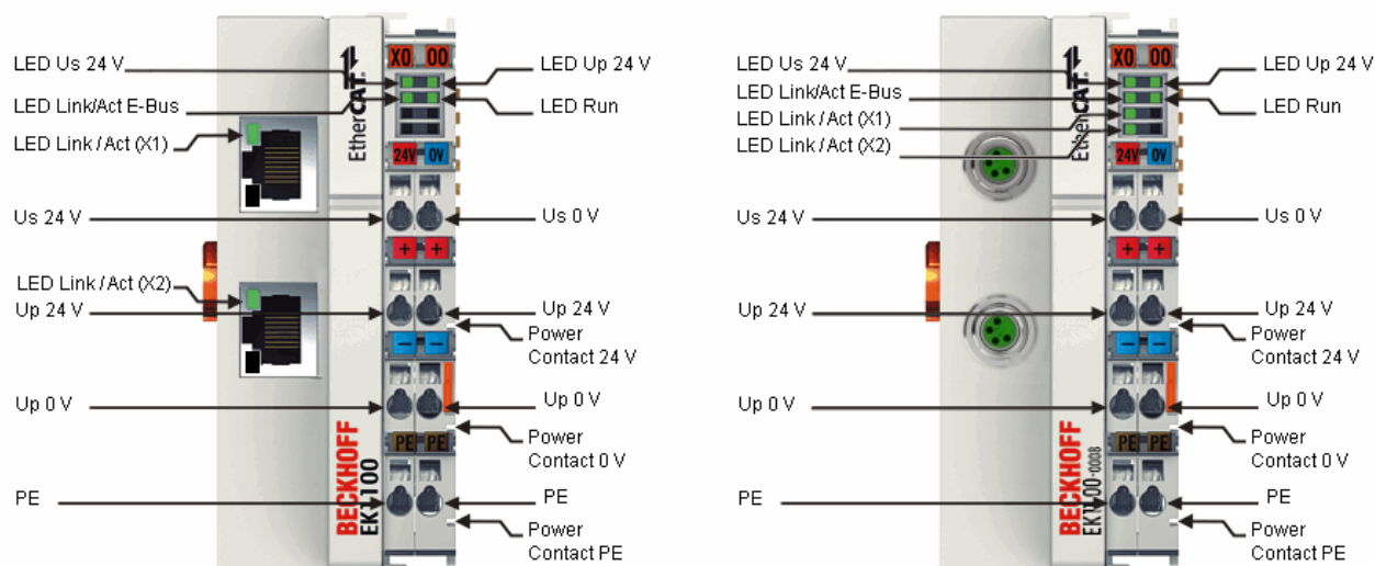
Abb. 61: Diagnose-LEDs EK1100, EK1100-0008
