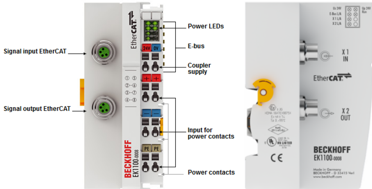
Abb. 18: EK1100-0008
