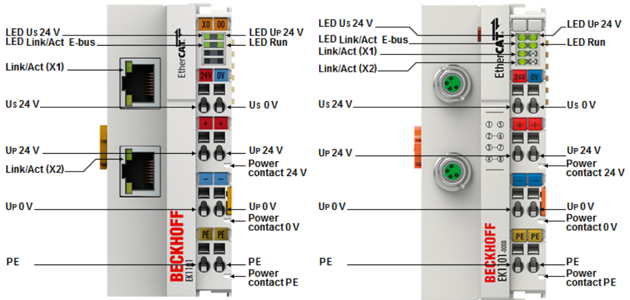
Abb. 62: Diagnose-LEDs EK1101-00x0, EK1101-0008
