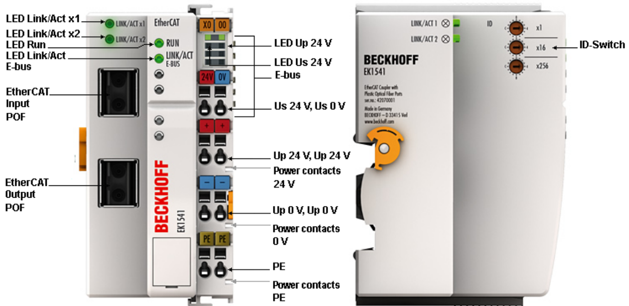
Abb. 51: EK1541
