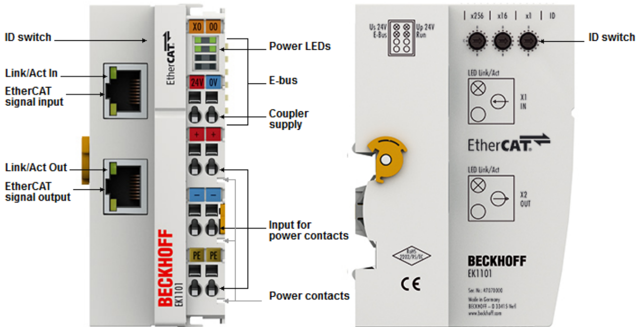
Abb. 6: EK1101
