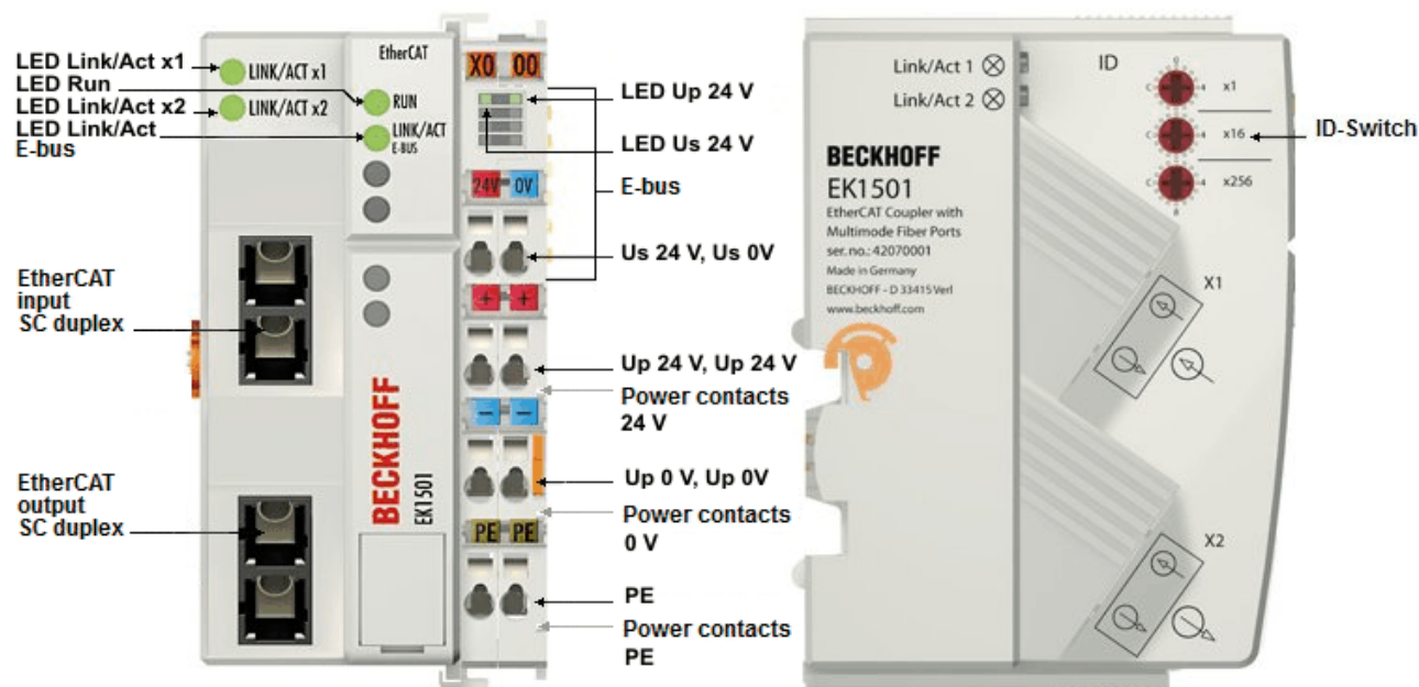
Abb. 63: Diagnose-LEDs Buskoppler EK15x1-00x0
