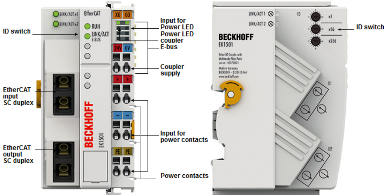
Abb. 20: EK1501
