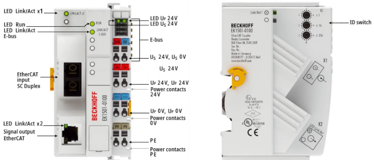
Abb. 64: Diagnose-LEDs Buskoppler EK1501-0100
